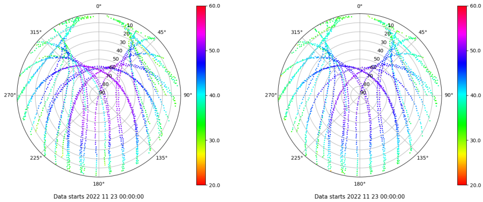
Skyplot for station VIGO. Signal to Noise S1C Data file VIGO00ESP_R_2022327.xtr Skyplot for station VIGO. Signal to Noise S2C Data file VIGO00ESP_R_2022327.xtr
