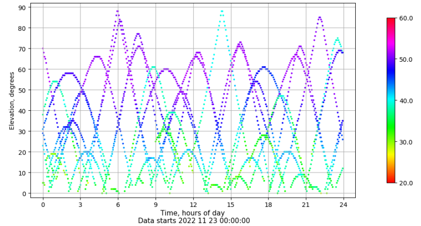
Time-elevation plot for station VIGO. Signal to Noise S1C Data file VIGO00ESP_R_2022327.xtr
