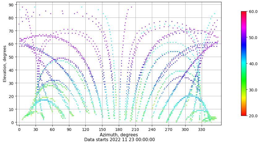
Azimuth-elevation plot for station VIGO. Signal to Noise S1C Data file VIGO00ESP_R_2022327.xtr
