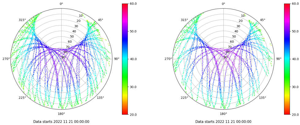
Skyplot for station VIGO. Signal to Noise S1C Data file VIGO00ESP_R_2022325.xtr Skyplot for station VIGO. Signal to Noise S2X Data file VIGO00ESP_R_2022325.xtr
