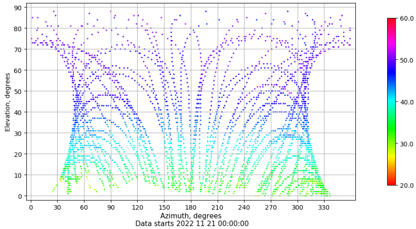
Azimuth-elevation plot for station VIGO. Signal to Noise S1C Data file VIGO00ESP_R_2022325.xtr
