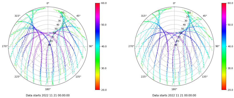
Skyplot for station VIGO. Signal to Noise S1C Data file VIGO00ESP_R_2022325.xtr Skyplot for station VIGO. Signal to Noise S2C Data file VIGO00ESP_R_2022325.xtr
