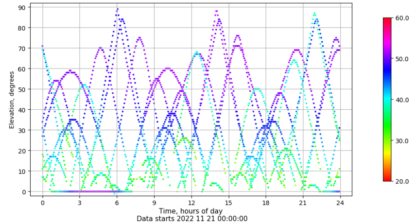
Time-elevation plot for station VIGO. Signal to Noise S1C Data file VIGO00ESP_R_2022325.xtr
