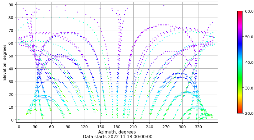
Azimuth-elevation plot for station VIGO. Signal to Noise S1C Data file VIGO00ESP_R_2022322.xtr
