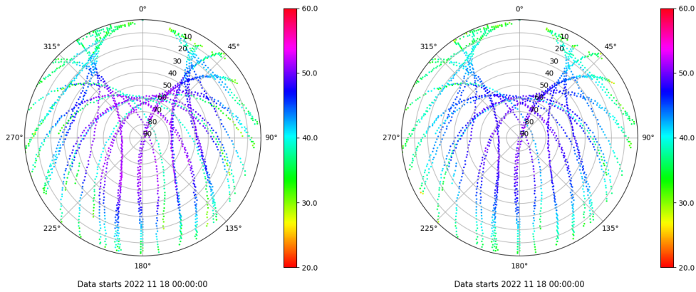
Skyplot for station VIGO. Signal to Noise S1C Data file VIGO00ESP_R_2022322.xtr Skyplot for station VIGO. Signal to Noise S2C Data file VIGO00ESP_R_2022322.xtr
