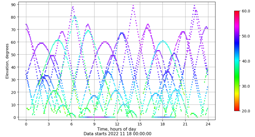
Time-elevation plot for station VIGO. Signal to Noise S1C Data file VIGO00ESP_R_2022322.xtr
