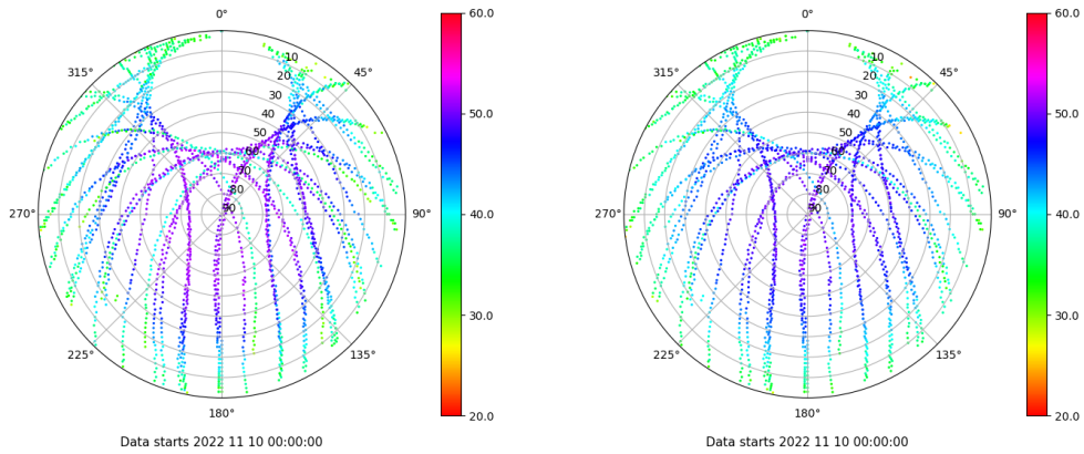
Skyplot for station VIGO. Signal to Noise S1C Data file VIGO00ESP_R_2022314.xtr Skyplot for station VIGO. Signal to Noise S2C Data file VIGO00ESP_R_2022314.xtr
