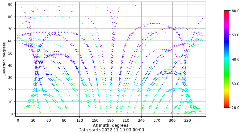
Azimuth-elevation plot for station VIGO. Signal to Noise S1C Data file VIGO00ESP_R_2022314.xtr
