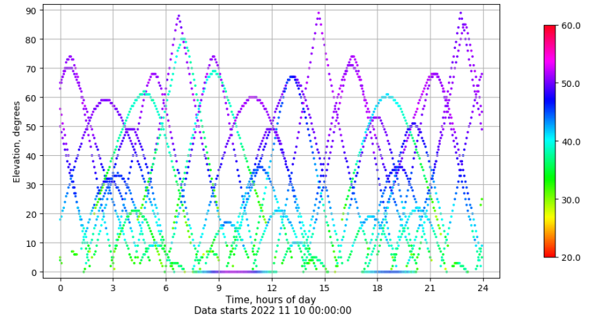
Time-elevation plot for station VIGO. Signal to Noise S1C Data file VIGO00ESP_R_2022314.xtr
