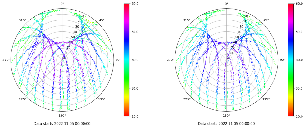
Skyplot for station VIGO. Signal to Noise S1C Data file VIGO00ESP_R_2022309.xtr Skyplot for station VIGO. Signal to Noise S2C Data file VIGO00ESP_R_2022309.xtr
