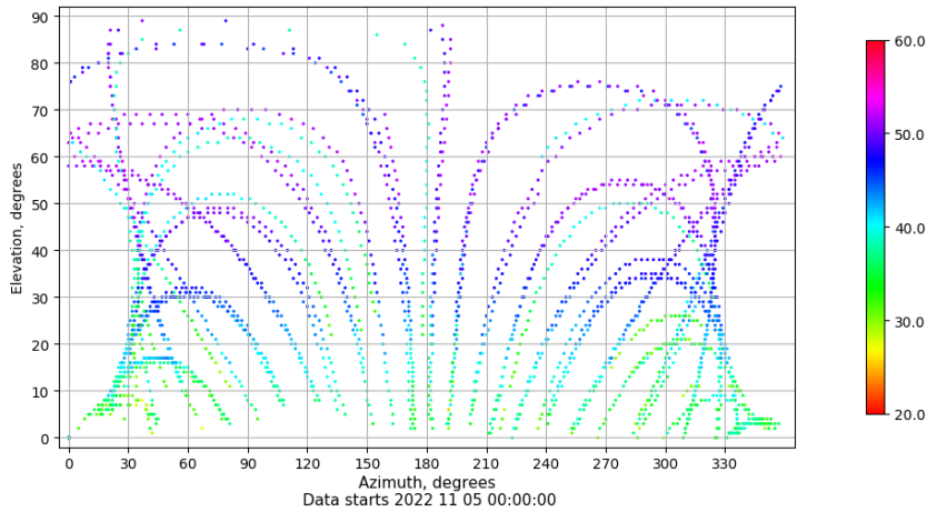
Azimuth-elevation plot for station VIGO. Signal to Noise S1C Data file VIGO00ESP_R_2022309.xtr
