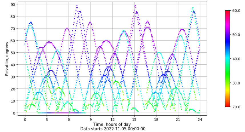
Time-elevation plot for station VIGO. Signal to Noise S1C Data file VIGO00ESP_R_2022309.xtr
