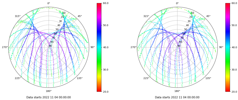
Skyplot for station VIGO. Signal to Noise S1C Data file VIGO00ESP_R_2022308.xtr Skyplot for station VIGO. Signal to Noise S2C Data file VIGO00ESP_R_2022308.xtr
