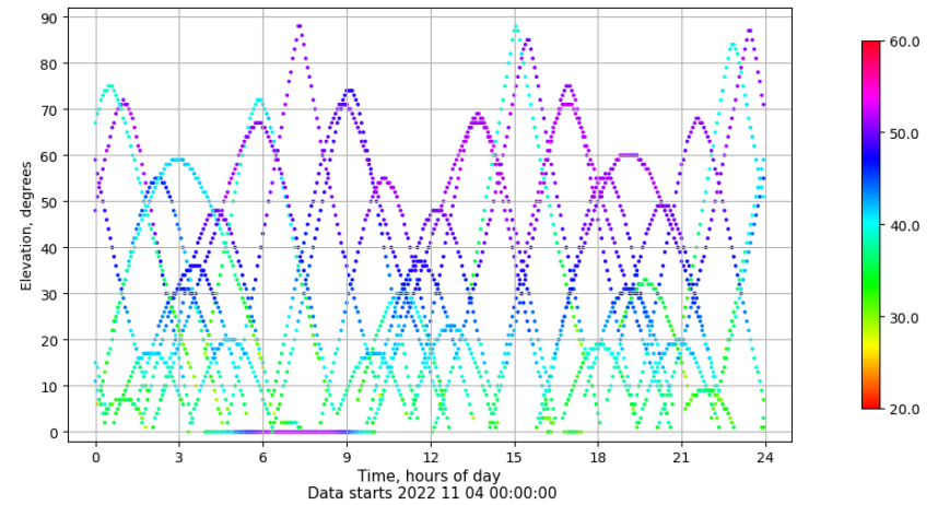
Time-elevation plot for station VIGO. Signal to Noise S1C Data file VIGO00ESP_R_2022308.xtr
