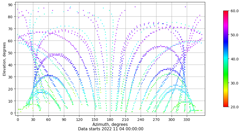
Azimuth-elevation plot for station VIGO. Signal to Noise S1C Data file VIGO00ESP_R_2022308.xtr
