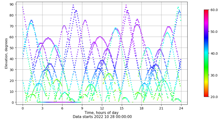
Time-elevation plot for station VIGO. Signal to Noise S1C Data file VIGO00ESP_R_2022301.xtr
