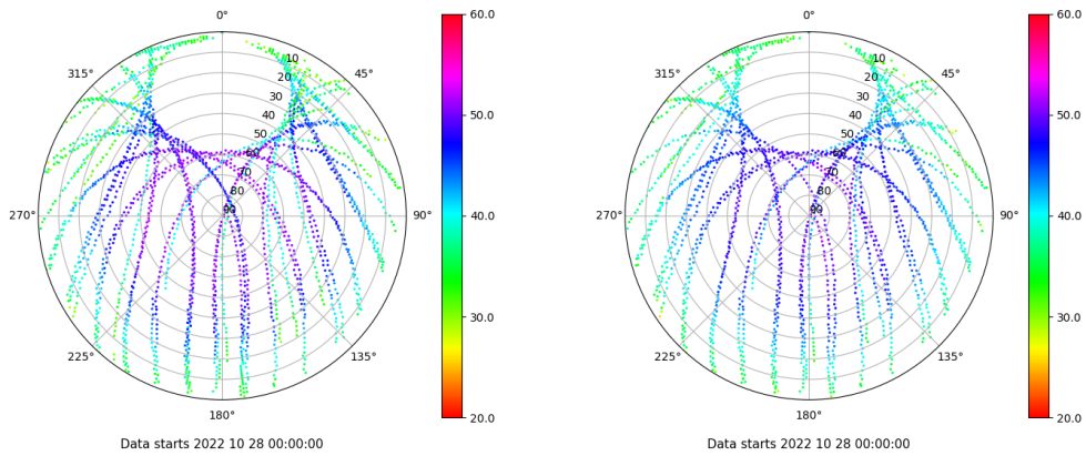
Skyplot for station VIGO. Signal to Noise S1C Data file VIGO00ESP_R_2022301.xtr Skyplot for station VIGO. Signal to Noise S2C Data file VIGO00ESP_R_2022301.xtr
