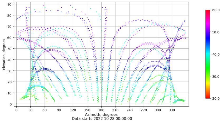
Azimuth-elevation plot for station VIGO. Signal to Noise S1C Data file VIGO00ESP_R_2022301.xtr
