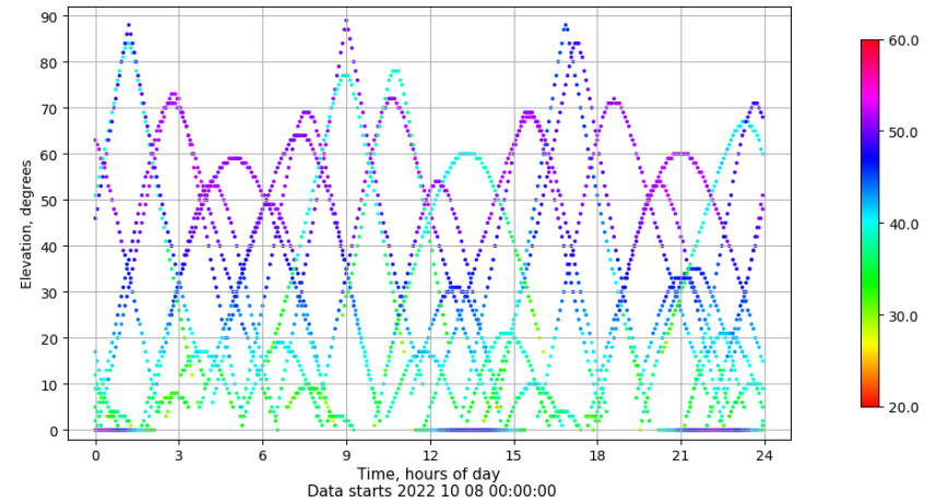
Time-elevation plot for station VIGO. Signal to Noise S1C Data file VIGO00ESP_R_2022281.xtr
