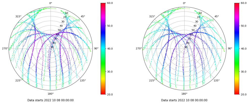
Skyplot for station VIGO. Signal to Noise S1C Data file VIGO00ESP_R_2022281.xtr Skyplot for station VIGO. Signal to Noise S2C Data file VIGO00ESP_R_2022281.xtr
