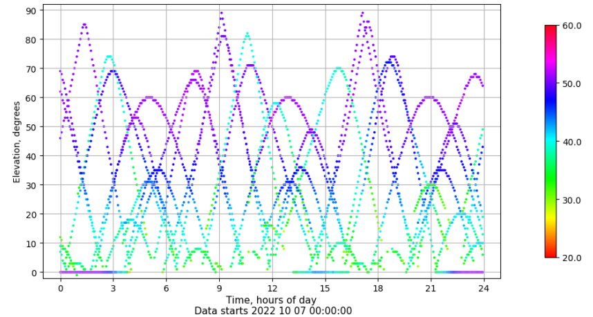
Time-elevation plot for station VIGO. Signal to Noise S1C Data file VIGO00ESP_R_2022280.xtr
