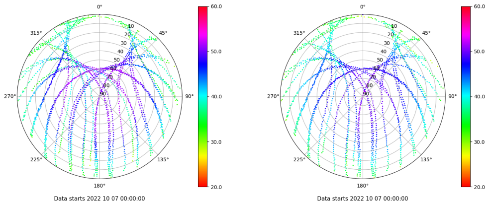
Skyplot for station VIGO. Signal to Noise S1C Data file VIGO00ESP_R_2022280.xtr Skyplot for station VIGO. Signal to Noise S2C Data file VIGO00ESP_R_2022280.xtr
