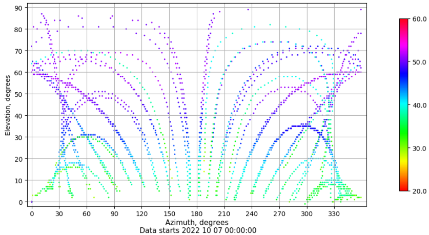
Azimuth-elevation plot for station VIGO. Signal to Noise S1C Data file VIGO00ESP_R_2022280.xtr
