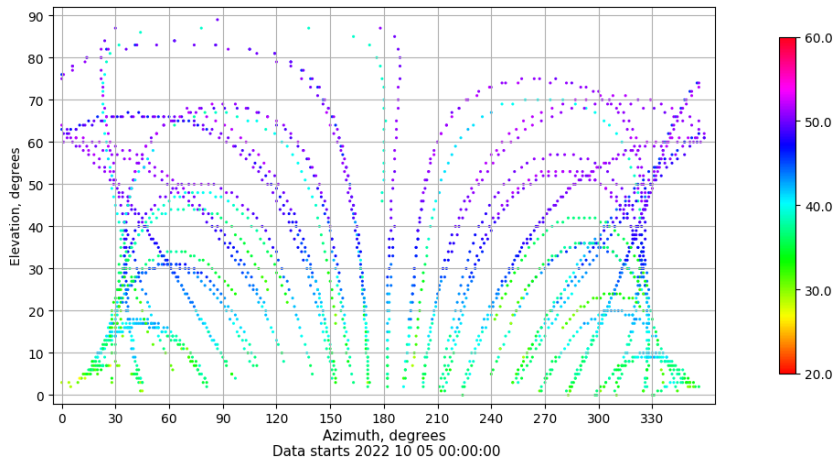
Azimuth-elevation plot for station VIGO. Signal to Noise S1C Data file VIGO00ESP_R_2022278.xtr
