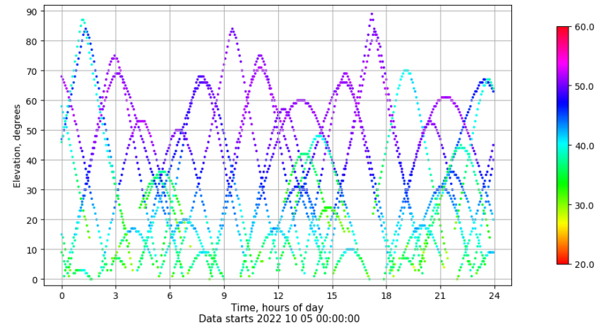
Time-elevation plot for station VIGO. Signal to Noise S1C Data file VIGO00ESP_R_2022278.xtr
