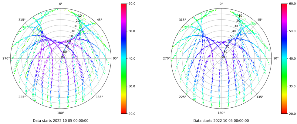
Skyplot for station VIGO. Signal to Noise S1C Data file VIGO00ESP_R_2022278.xtr Skyplot for station VIGO. Signal to Noise S2C Data file VIGO00ESP_R_2022278.xtr
