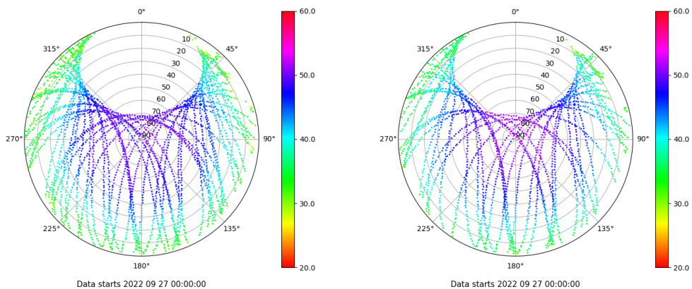
Skyplot for station VIGO. Signal to Noise S1C Data file VIGO00ESP_R_2022270.xtr Skyplot for station VIGO. Signal to Noise S2X Data file VIGO00ESP_R_2022270.xtr
