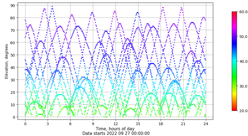
Time-elevation plot for station VIGO. Signal to Noise S1C Data file VIGO00ESP_R_2022270.xtr
