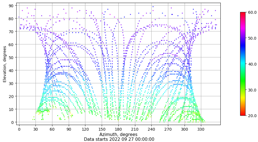
Azimuth-elevation plot for station VIGO. Signal to Noise S1C Data file VIGO00ESP_R_2022270.xtr
