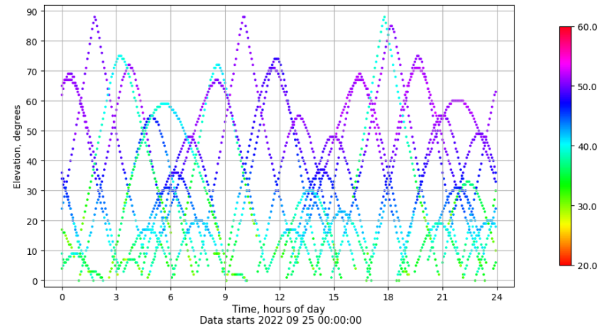
Time-elevation plot for station VIGO. Signal to Noise S1C Data file VIGO00ESP_R_2022268.xtr
