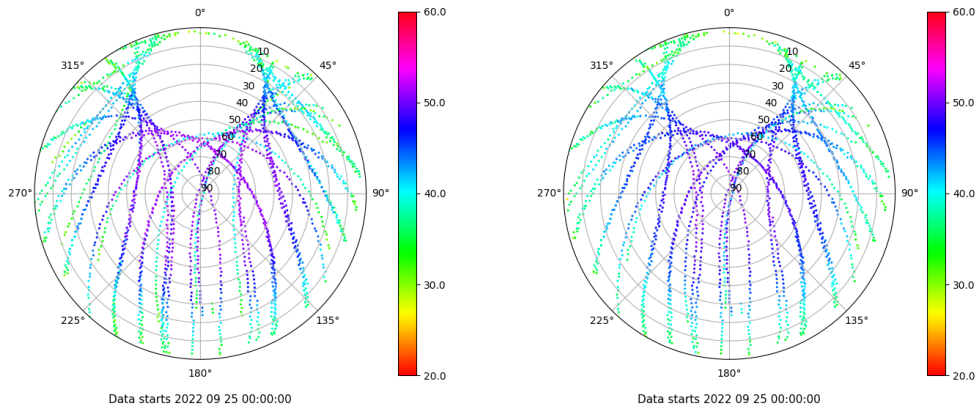
Skyplot for station VIGO. Signal to Noise S1C Data file VIGO00ESP_R_2022268.xtr Skyplot for station VIGO. Signal to Noise S2C Data file VIGO00ESP_R_2022268.xtr
