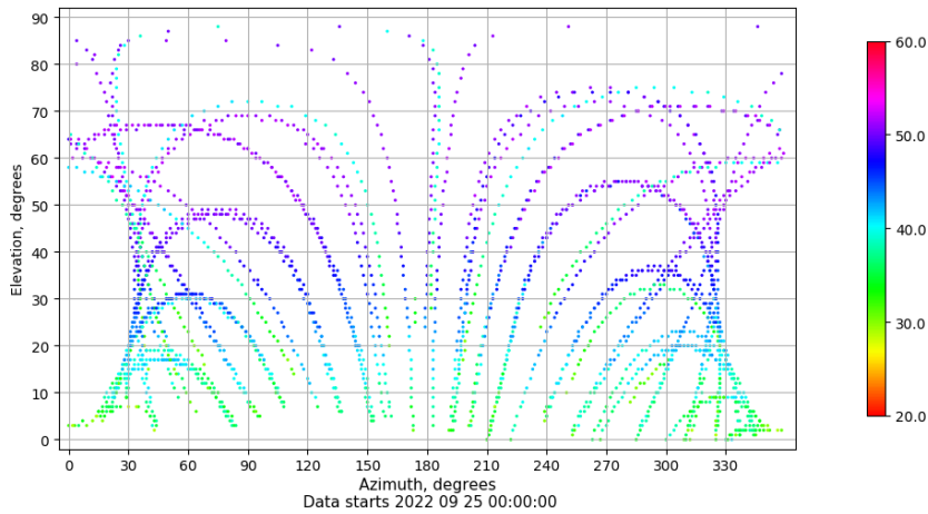
Azimuth-elevation plot for station VIGO. Signal to Noise S1C Data file VIGO00ESP_R_2022268.xtr
