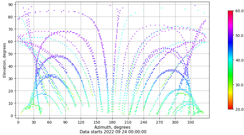
Azimuth-elevation plot for station VIGO. Signal to Noise S1C Data file VIGO00ESP_R_2022267.xtr
