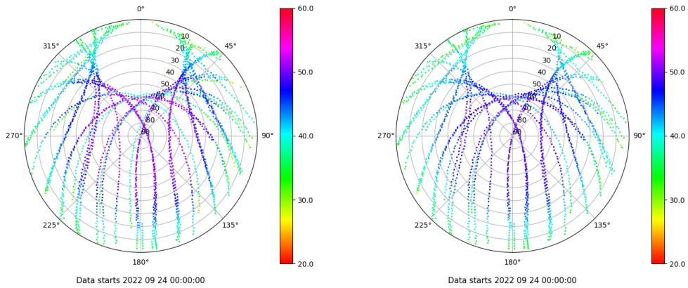
Skyplot for station VIGO. Signal to Noise S1C Data file VIGO00ESP_R_2022267.xtr Skyplot for station VIGO. Signal to Noise S2C Data file VIGO00ESP_R_2022267.xtr
