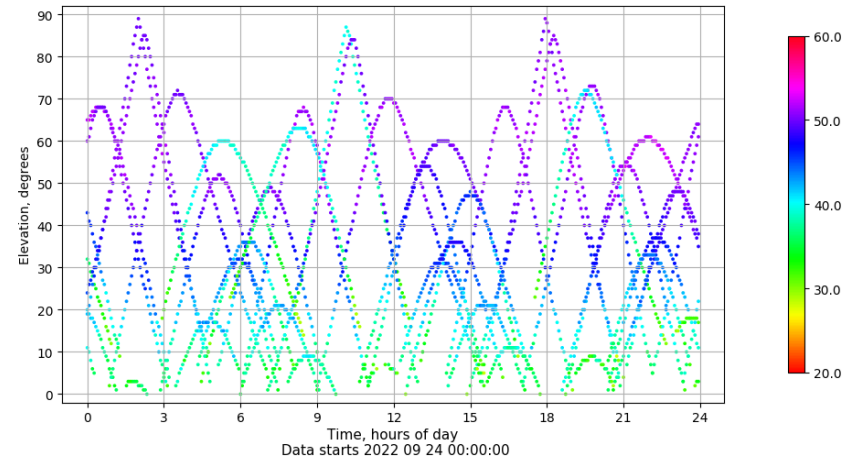
Time-elevation plot for station VIGO. Signal to Noise S1C Data file VIGO00ESP_R_2022267.xtr
