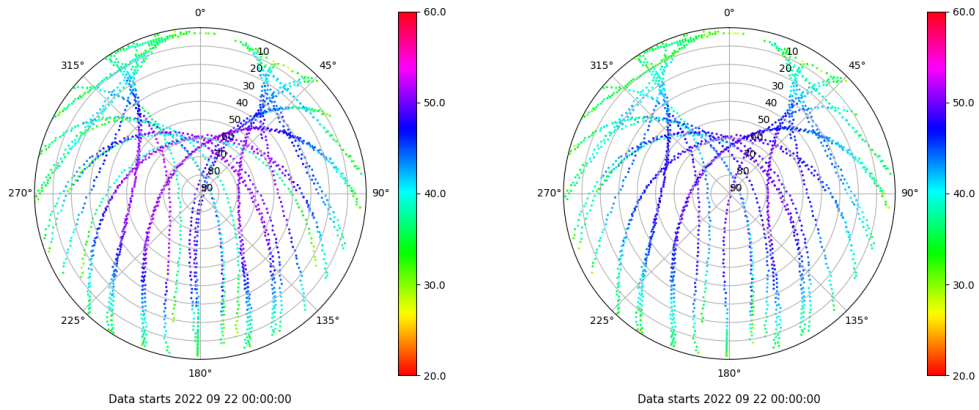
Skyplot for station VIGO. Signal to Noise S1C Data file VIGO00ESP_R_2022265.xtr Skyplot for station VIGO. Signal to Noise S2C Data file VIGO00ESP_R_2022265.xtr
