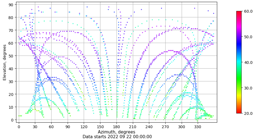
Azimuth-elevation plot for station VIGO. Signal to Noise S1C Data file VIGO00ESP_R_2022265.xtr
