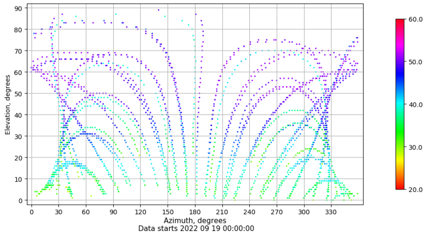
Azimuth-elevation plot for station VIGO. Signal to Noise S1C Data file VIGO00ESP_R_2022262.xtr
