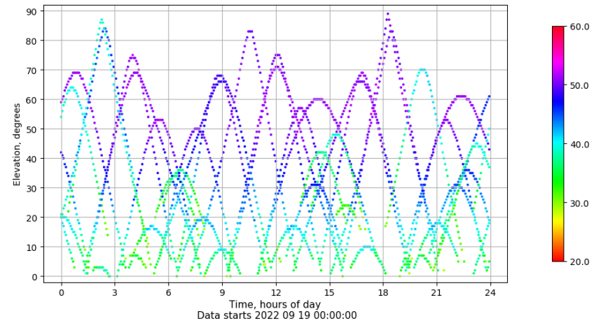
Time-elevation plot for station VIGO. Signal to Noise S1C Data file VIGO00ESP_R_2022262.xtr
