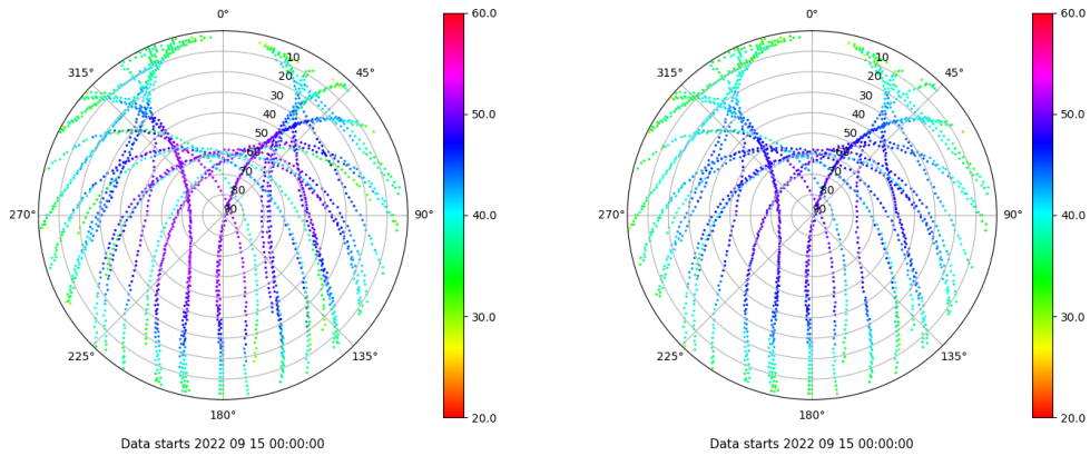
Skyplot for station VIGO. Signal to Noise S1C Data file VIGO00ESP_R_2022258.xtr Skyplot for station VIGO. Signal to Noise S2C Data file VIGO00ESP_R_2022258.xtr
