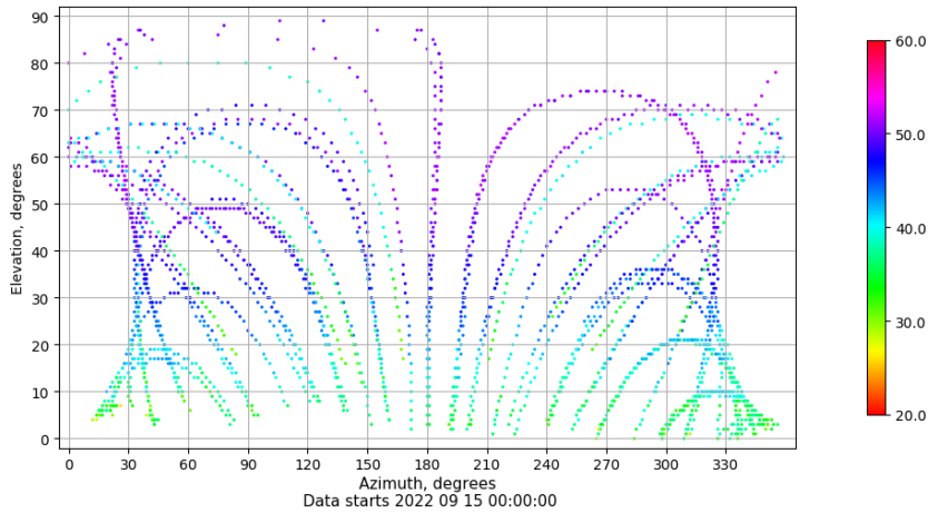
Azimuth-elevation plot for station VIGO. Signal to Noise S1C Data file VIGO00ESP_R_2022258.xtr
