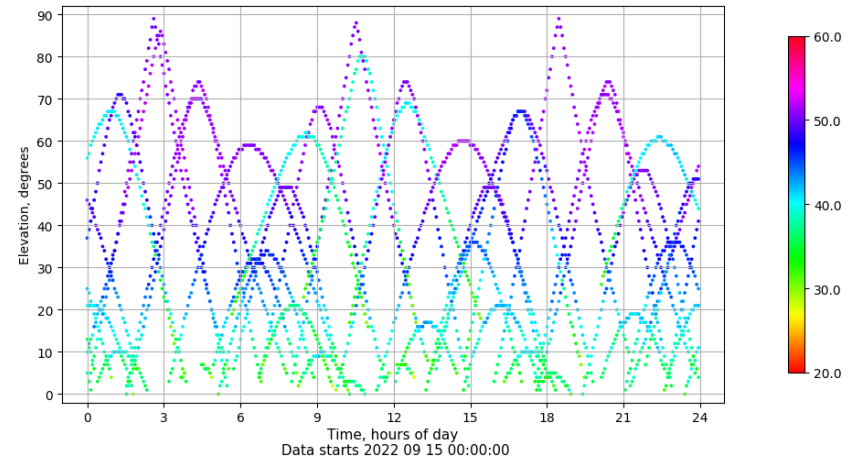
Time-elevation plot for station VIGO. Signal to Noise S1C Data file VIGO00ESP_R_2022258.xtr
