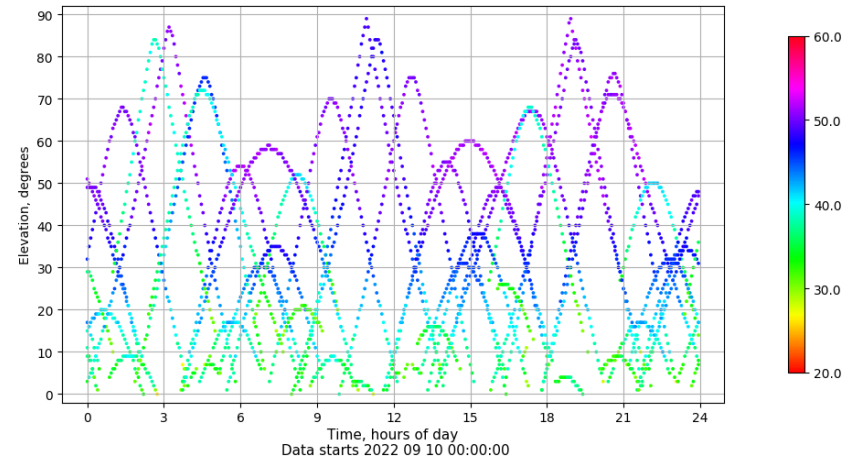
Time-elevation plot for station VIGO. Signal to Noise S1C Data file VIGO00ESP_R_2022253.xtr
