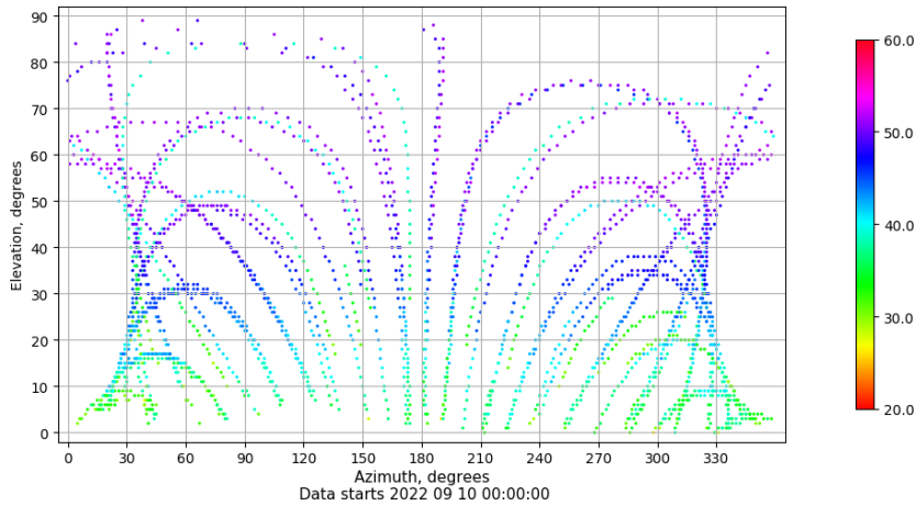
Azimuth-elevation plot for station VIGO. Signal to Noise S1C Data file VIGO00ESP_R_2022253.xtr
