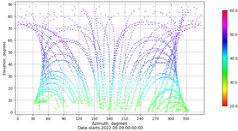
Azimuth-elevation plot for station VIGO. Signal to Noise S1C Data file VIGO00ESP_R_2022252.xtr
