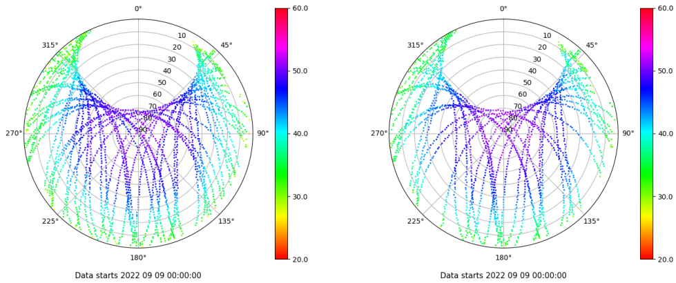
Skyplot for station VIGO. Signal to Noise S1C Data file VIGO00ESP_R_2022252.xtr Skyplot for station VIGO. Signal to Noise S2X Data file VIGO00ESP_R_2022252.xtr
