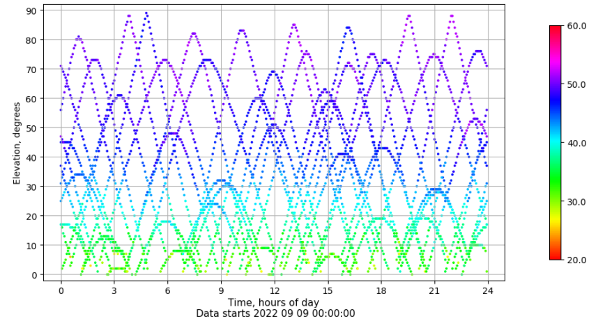
Time-elevation plot for station VIGO. Signal to Noise S1C Data file VIGO00ESP_R_2022252.xtr
