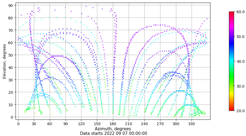
Azimuth-elevation plot for station VIGO. Signal to Noise S1C Data file VIGO00ESP_R_2022250.xtr
