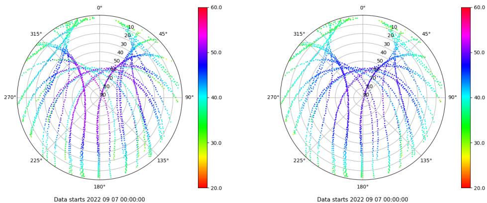
Skyplot for station VIGO. Signal to Noise S1C Data file VIGO00ESP_R_2022250.xtr Skyplot for station VIGO. Signal to Noise S2C Data file VIGO00ESP_R_2022250.xtr
