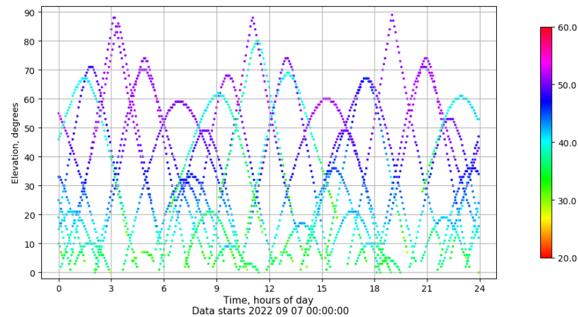
Time-elevation plot for station VIGO. Signal to Noise S1C Data file VIGO00ESP_R_2022250.xtr
