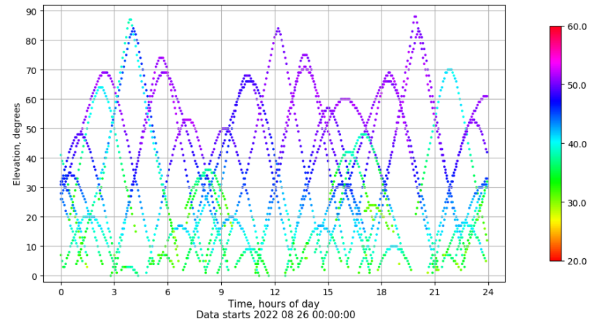
Time-elevation plot for station VIGO. Signal to Noise S1C Data file VIGO00ESP_R_2022238.xtr
