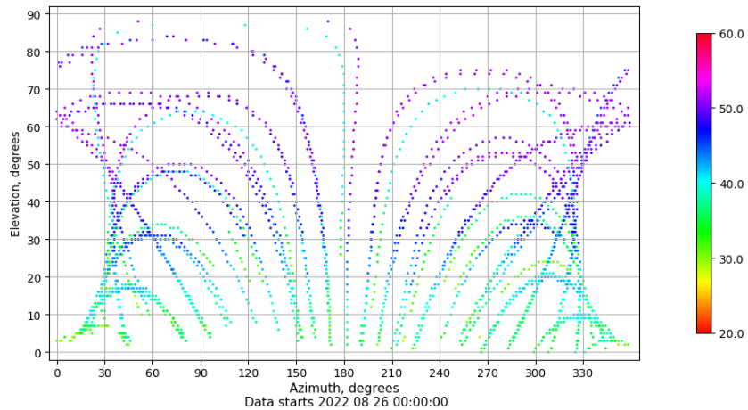
Azimuth-elevation plot for station VIGO. Signal to Noise S1C Data file VIGO00ESP_R_2022238.xtr
