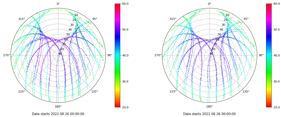
Skyplot for station VIGO. Signal to Noise S1C Data file VIGO00ESP_R_2022238.xtr Skyplot for station VIGO. Signal to Noise S2C Data file VIGO00ESP_R_2022238.xtr
