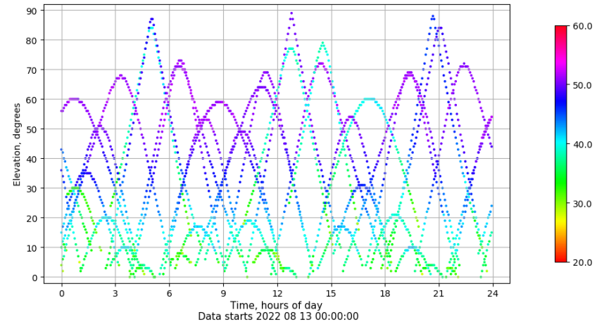
Time-elevation plot for station VIGO. Signal to Noise S1C Data file VIGO00ESP_R_2022225.xtr
