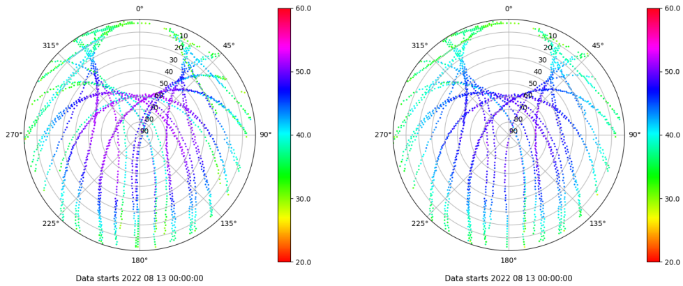
Skyplot for station VIGO. Signal to Noise S1C Data file VIGO00ESP_R_2022225.xtr Skyplot for station VIGO. Signal to Noise S2C Data file VIGO00ESP_R_2022225.xtr
