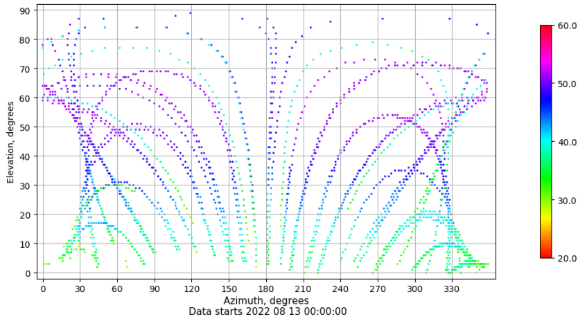
Azimuth-elevation plot for station VIGO. Signal to Noise S1C Data file VIGO00ESP_R_2022225.xtr
