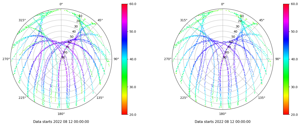
Skyplot for station VIGO. Signal to Noise S1C Data file VIGO00ESP_R_2022224.xtr Skyplot for station VIGO. Signal to Noise S2C Data file VIGO00ESP_R_2022224.xtr
