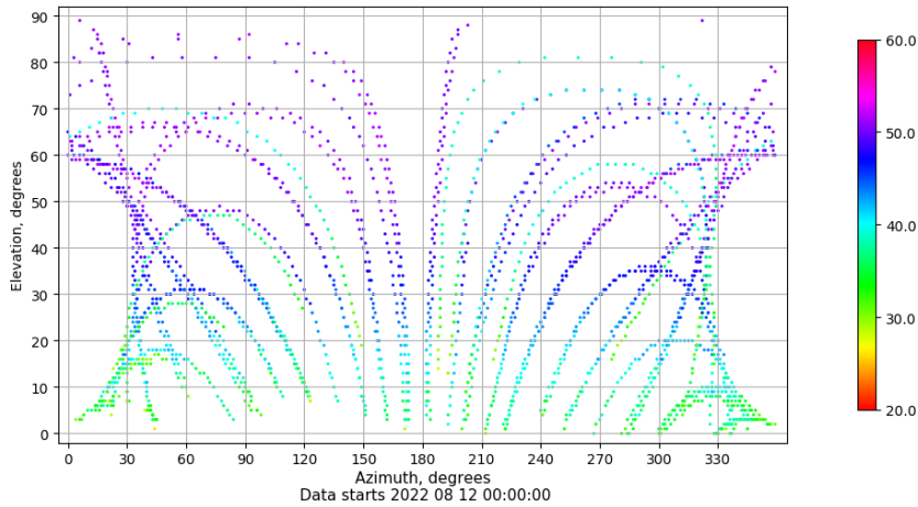
Azimuth-elevation plot for station VIGO. Signal to Noise S1C Data file VIGO00ESP_R_2022224.xtr
