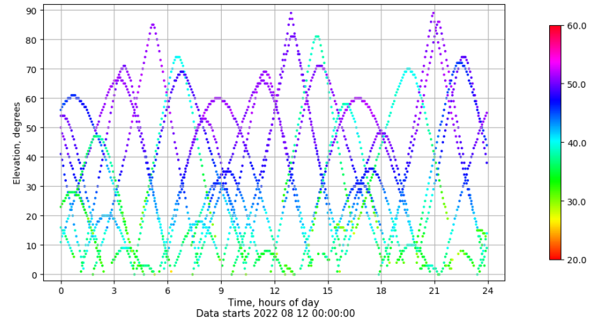
Time-elevation plot for station VIGO. Signal to Noise S1C Data file VIGO00ESP_R_2022224.xtr
