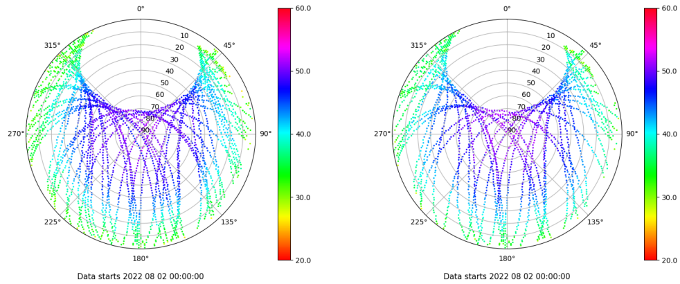
Skyplot for station VIGO. Signal to Noise S1C Data file VIGO00ESP_R_2022214.xtr Skyplot for station VIGO. Signal to Noise S2X Data file VIGO00ESP_R_2022214.xtr
