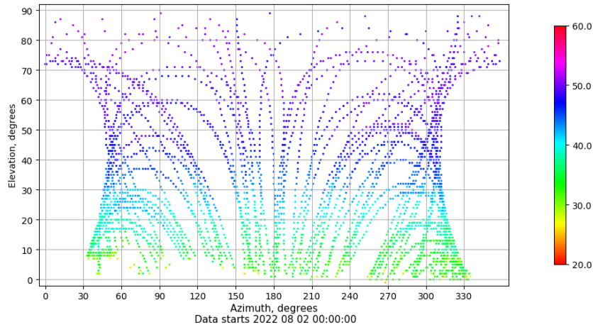
Azimuth-elevation plot for station VIGO. Signal to Noise S1C Data file VIGO00ESP_R_2022214.xtr
