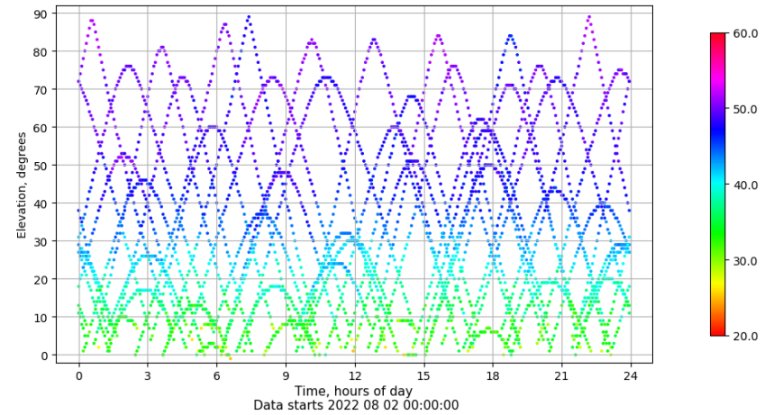
Time-elevation plot for station VIGO. Signal to Noise S1C Data file VIGO00ESP_R_2022214.xtr
