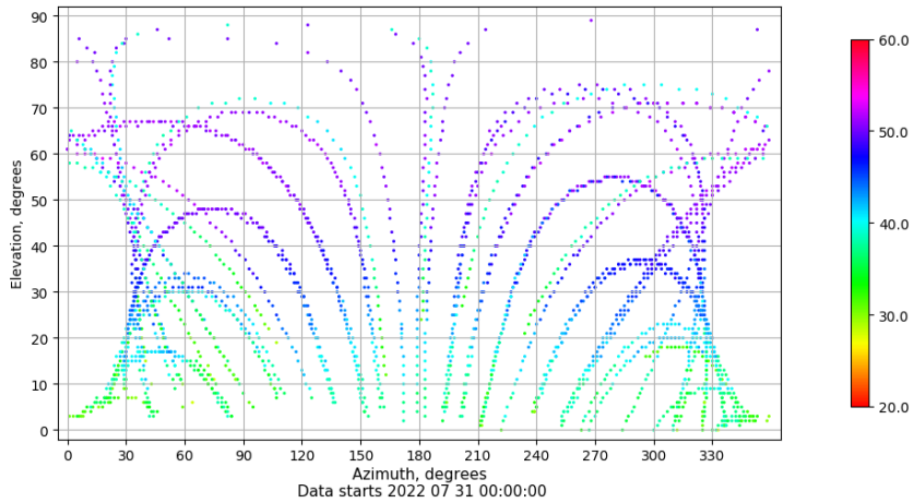
Azimuth-elevation plot for station VIGO. Signal to Noise S1C Data file VIGO00ESP_R_2022212.xtr
