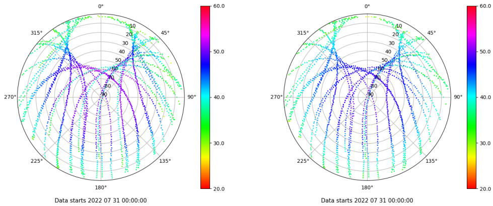
Skyplot for station VIGO. Signal to Noise S1C Data file VIGO00ESP_R_2022212.xtr Skyplot for station VIGO. Signal to Noise S2C Data file VIGO00ESP_R_2022212.xtr
