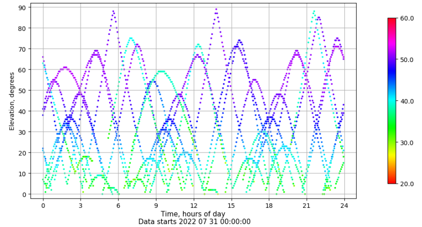
Time-elevation plot for station VIGO. Signal to Noise S1C Data file VIGO00ESP_R_2022212.xtr
