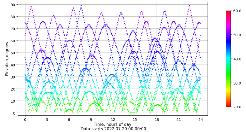
Time-elevation plot for station VIGO. Signal to Noise S1C Data file VIGO00ESP_R_2022210.xtr
