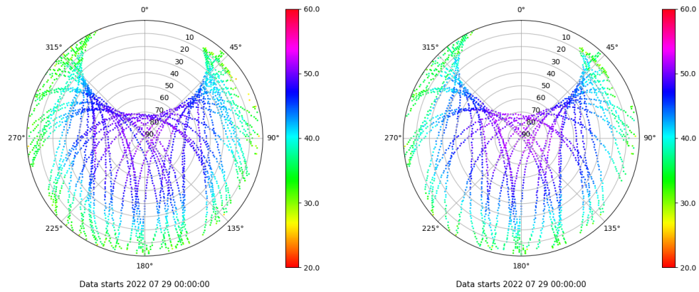
Skyplot for station VIGO. Signal to Noise S1C Data file VIGO00ESP_R_2022210.xtr Skyplot for station VIGO. Signal to Noise S2X Data file VIGO00ESP_R_2022210.xtr
