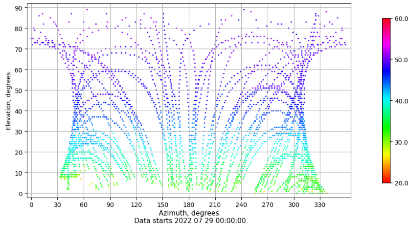
Azimuth-elevation plot for station VIGO. Signal to Noise S1C Data file VIGO00ESP_R_2022210.xtr
