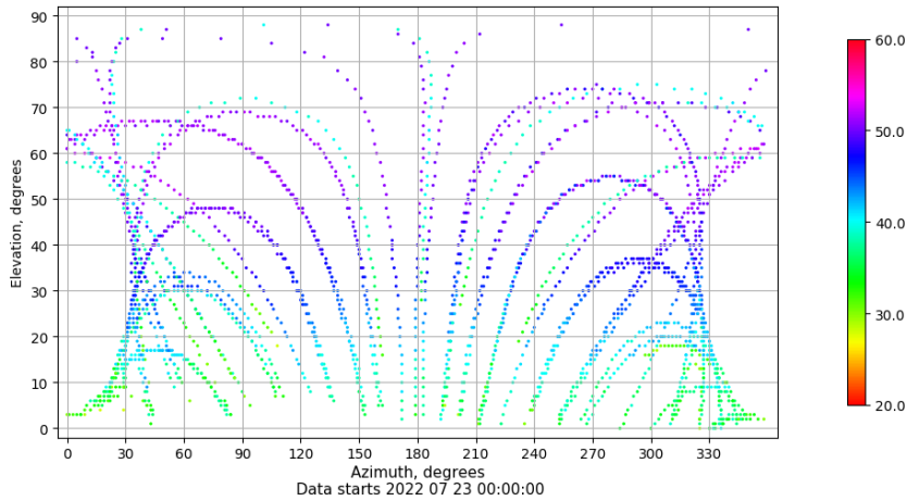
Azimuth-elevation plot for station VIGO. Signal to Noise S1C Data file VIGO00ESP_R_2022204.xtr
