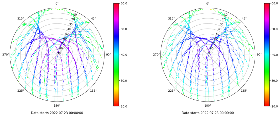
Skyplot for station VIGO. Signal to Noise S1C Data file VIGO00ESP_R_2022204.xtr Skyplot for station VIGO. Signal to Noise S2C Data file VIGO00ESP_R_2022204.xtr
