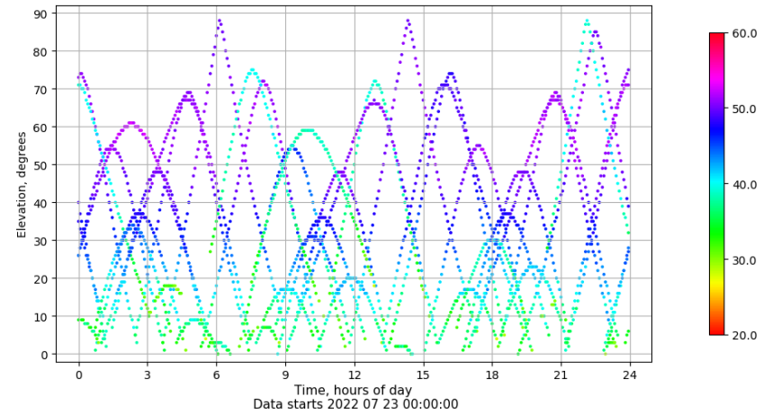
Time-elevation plot for station VIGO. Signal to Noise S1C Data file VIGO00ESP_R_2022204.xtr
