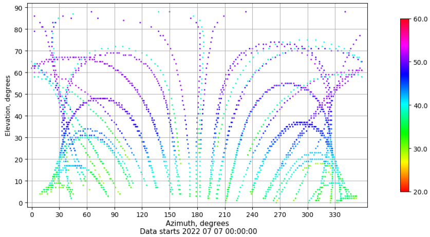
Azimuth-elevation plot for station VIGO. Signal to Noise S1C Data file VIGO00ESP_R_2022188.xtr
