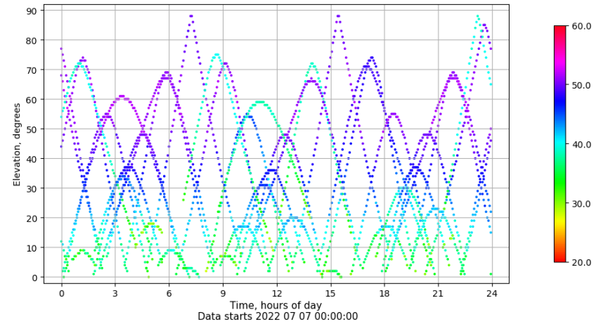
Time-elevation plot for station VIGO. Signal to Noise S1C Data file VIGO00ESP_R_2022188.xtr
