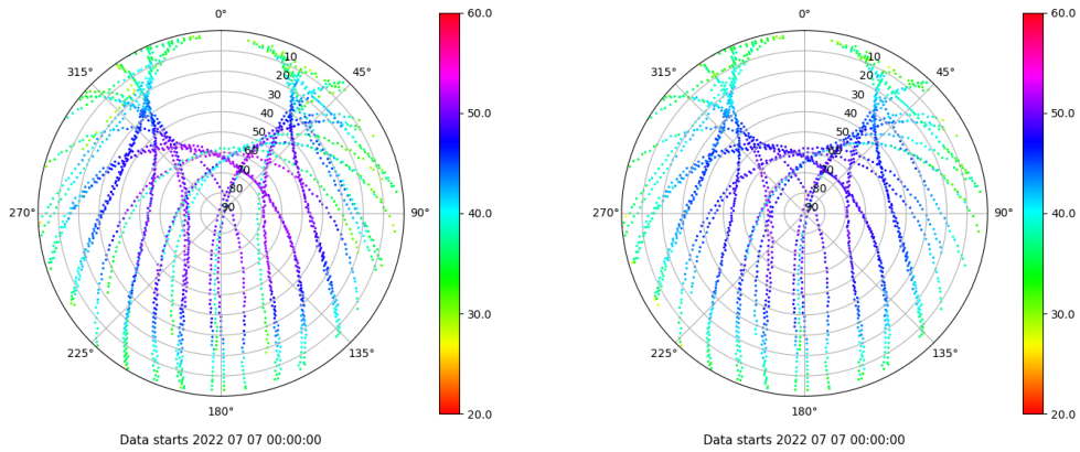
Skyplot for station VIGO. Signal to Noise S1C Data file VIGO00ESP_R_2022188.xtr Skyplot for station VIGO. Signal to Noise S2C Data file VIGO00ESP_R_2022188.xtr
