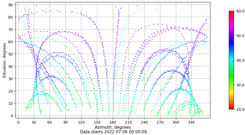
Azimuth-elevation plot for station VIGO. Signal to Noise S1C Data file VIGO00ESP_R_2022187.xtr
