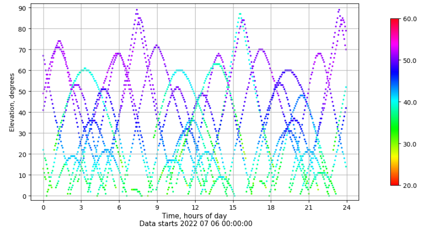
Time-elevation plot for station VIGO. Signal to Noise S1C Data file VIGO00ESP_R_2022187.xtr
