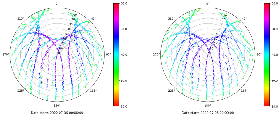
Skyplot for station VIGO. Signal to Noise S1C Data file VIGO00ESP_R_2022187.xtr Skyplot for station VIGO. Signal to Noise S2C Data file VIGO00ESP_R_2022187.xtr
