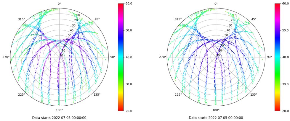
Skyplot for station VIGO. Signal to Noise S1C Data file VIGO00ESP_R_2022186.xtr Skyplot for station VIGO. Signal to Noise S2C Data file VIGO00ESP_R_2022186.xtr
