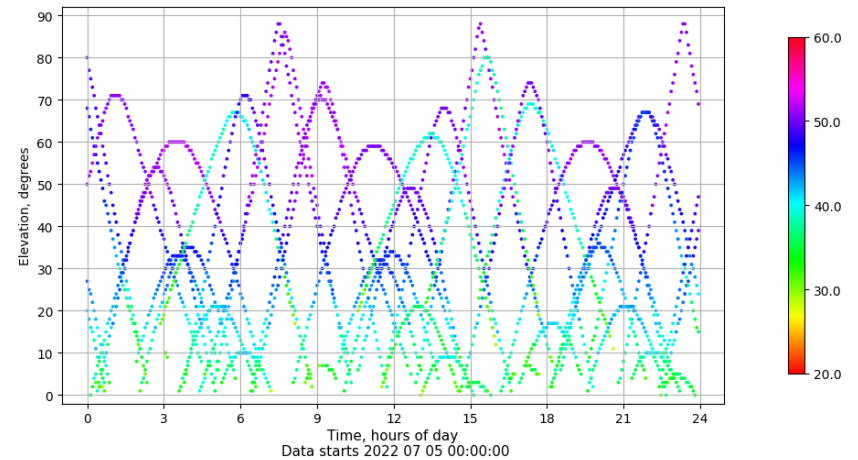
Time-elevation plot for station VIGO. Signal to Noise S1C Data file VIGO00ESP_R_2022186.xtr
