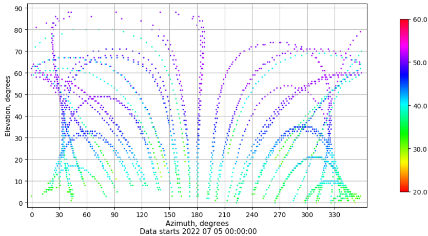
Azimuth-elevation plot for station VIGO. Signal to Noise S1C Data file VIGO00ESP_R_2022186.xtr
