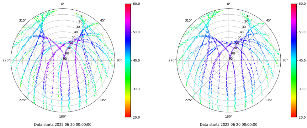
Skyplot for station VIGO. Signal to Noise S1C Data file VIGO00ESP_R_2022171.xtr Skyplot for station VIGO. Signal to Noise S2C Data file VIGO00ESP_R_2022171.xtr
