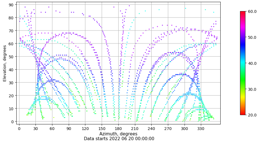
Azimuth-elevation plot for station VIGO. Signal to Noise S1C Data file VIGO00ESP_R_2022171.xtr
