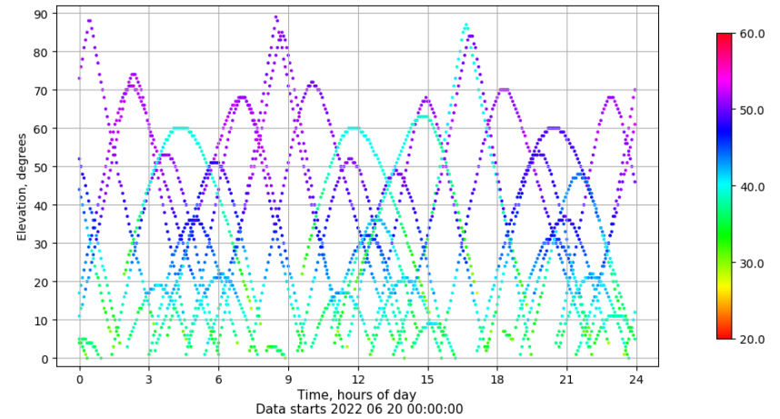
Time-elevation plot for station VIGO. Signal to Noise S1C Data file VIGO00ESP_R_2022171.xtr
