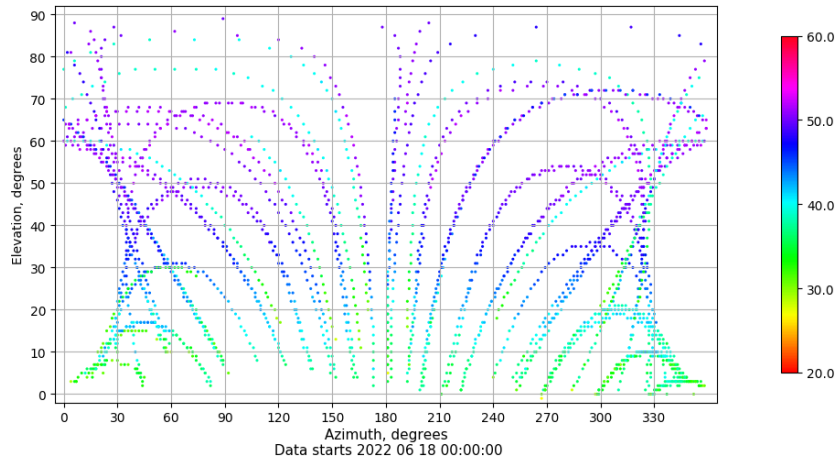
Azimuth-elevation plot for station VIGO. Signal to Noise S1C Data file VIGO00ESP_R_2022169.xtr
