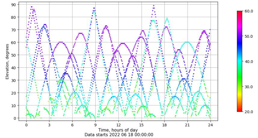
Time-elevation plot for station VIGO. Signal to Noise S1C Data file VIGO00ESP_R_2022169.xtr
