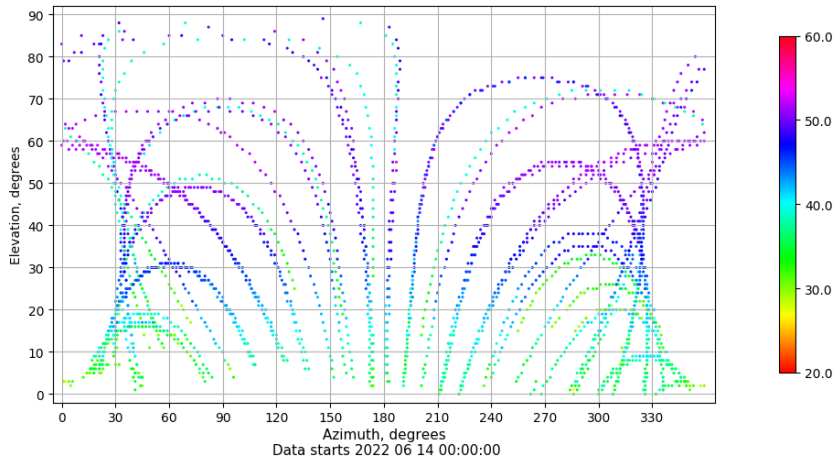
Azimuth-elevation plot for station VIGO. Signal to Noise S1C Data file VIGO00ESP_R_2022165.xtr
