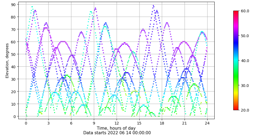
Time-elevation plot for station VIGO. Signal to Noise S1C Data file VIGO00ESP_R_2022165.xtr
