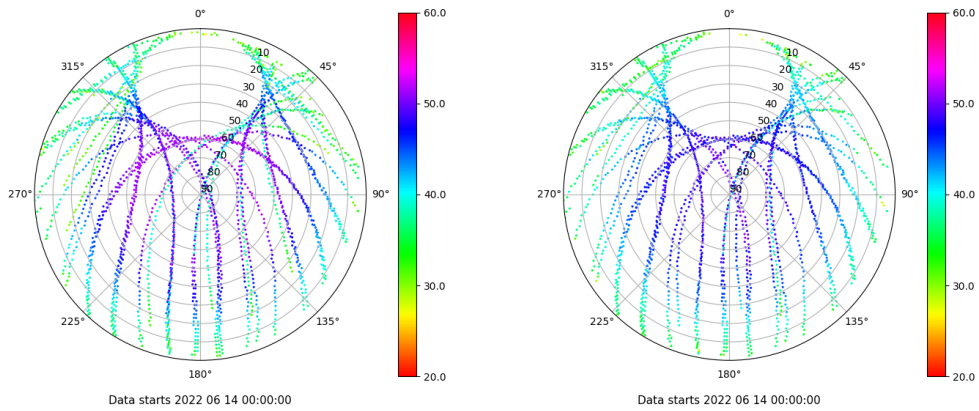
Skyplot for station VIGO. Signal to Noise S1C Data file VIGO00ESP_R_2022165.xtr Skyplot for station VIGO. Signal to Noise S2C Data file VIGO00ESP_R_2022165.xtr
