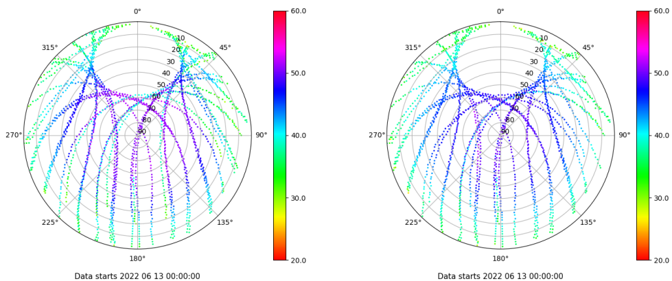
Skyplot for station VIGO. Signal to Noise S1C Data file VIGO00ESP_R_2022164.xtr Skyplot for station VIGO. Signal to Noise S2C Data file VIGO00ESP_R_2022164.xtr
