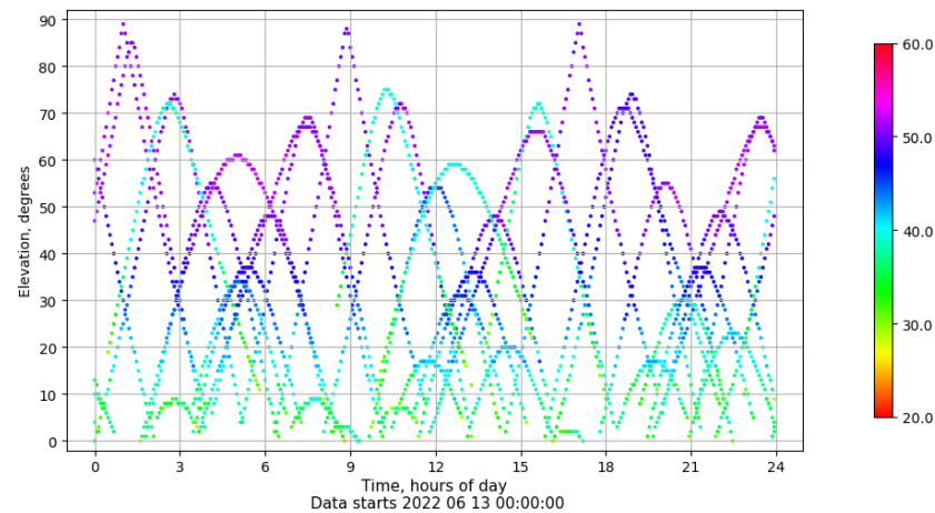
Time-elevation plot for station VIGO. Signal to Noise S1C Data file VIGO00ESP_R_2022164.xtr
