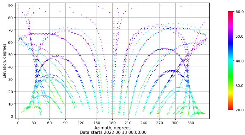
Azimuth-elevation plot for station VIGO. Signal to Noise S1C Data file VIGO00ESP_R_2022164.xtr
