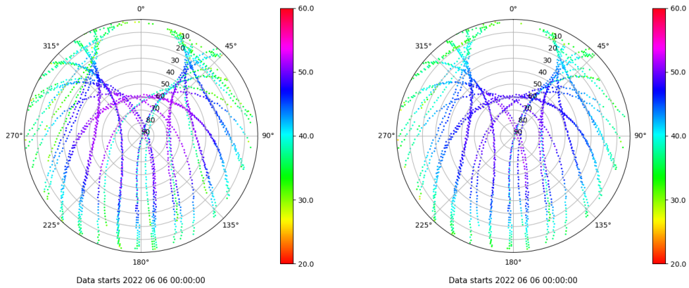
Skyplot for station VIGO. Signal to Noise S1C Data file VIGO00ESP_R_2022157.xtr Skyplot for station VIGO. Signal to Noise S2C Data file VIGO00ESP_R_2022157.xtr
