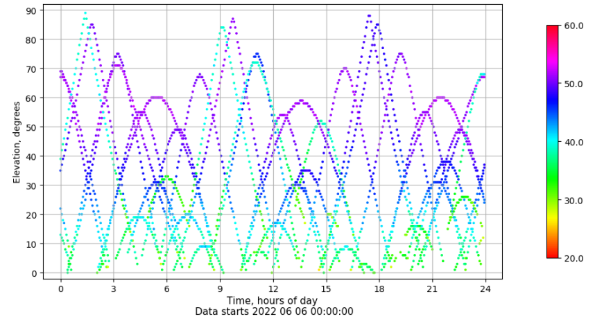
Time-elevation plot for station VIGO. Signal to Noise S1C Data file VIGO00ESP_R_2022157.xtr
