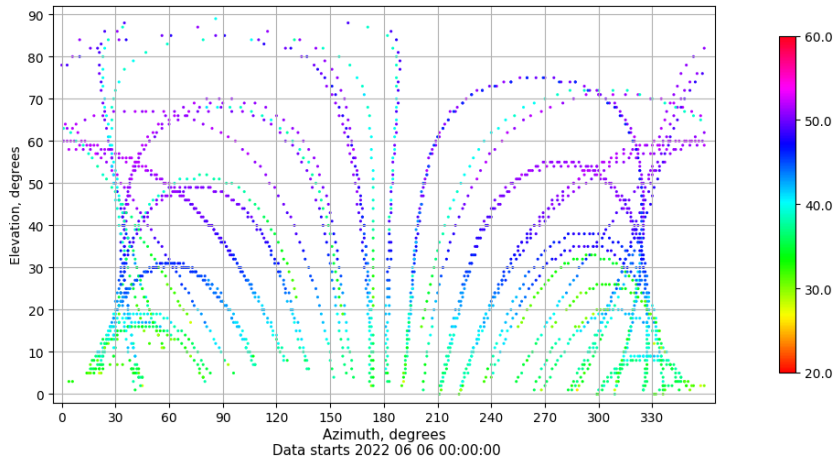
Azimuth-elevation plot for station VIGO. Signal to Noise S1C Data file VIGO00ESP_R_2022157.xtr
