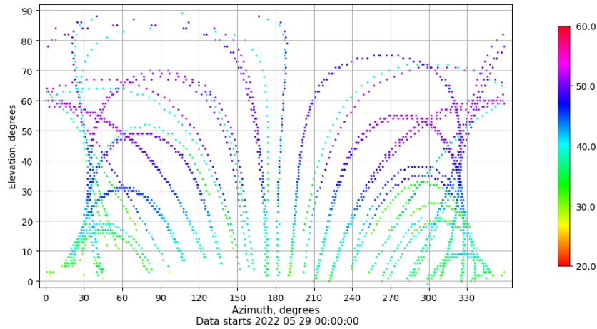
Azimuth-elevation plot for station VIGO. Signal to Noise S1C Data file VIGO00ESP_R_2022149.xtr
