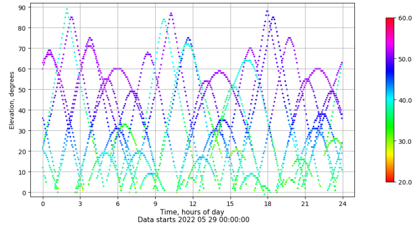
Time-elevation plot for station VIGO. Signal to Noise S1C Data file VIGO00ESP_R_2022149.xtr
