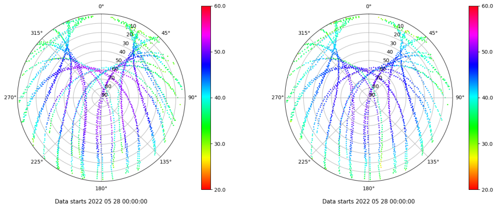
Skyplot for station VIGO. Signal to Noise S1C Data file VIGO00ESP_R_2022148.xtr Skyplot for station VIGO. Signal to Noise S2C Data file VIGO00ESP_R_2022148.xtr
