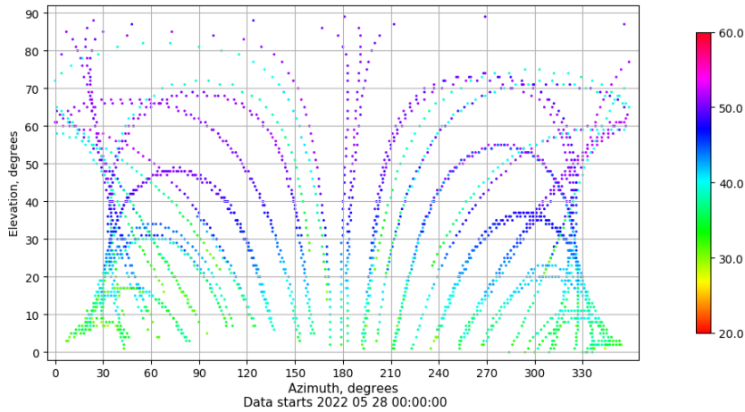
Azimuth-elevation plot for station VIGO. Signal to Noise S1C Data file VIGO00ESP_R_2022148.xtr
