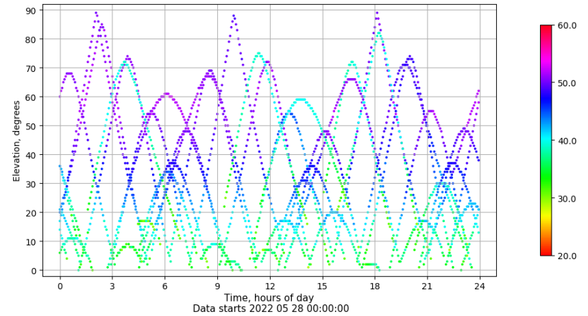
Time-elevation plot for station VIGO. Signal to Noise S1C Data file VIGO00ESP_R_2022148.xtr
