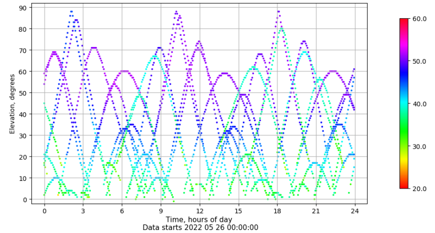
Time-elevation plot for station VIGO. Signal to Noise S1C Data file VIGO00ESP_R_2022146.xtr
