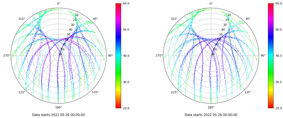
Skyplot for station VIGO. Signal to Noise S1C Data file VIGO00ESP_R_2022146.xtr Skyplot for station VIGO. Signal to Noise S2C Data file VIGO00ESP_R_2022146.xtr
