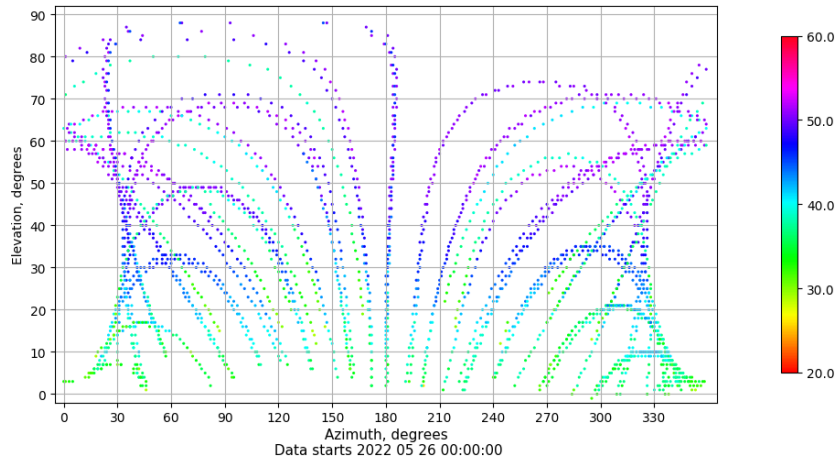
Azimuth-elevation plot for station VIGO. Signal to Noise S1C Data file VIGO00ESP_R_2022146.xtr
