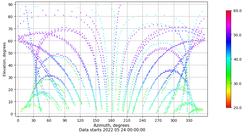
Azimuth-elevation plot for station VIGO. Signal to Noise S1C Data file VIGO00ESP_R_2022144.xtr
