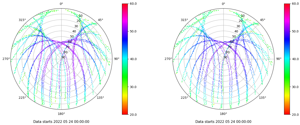
Skyplot for station VIGO. Signal to Noise S1C Data file VIGO00ESP_R_2022144.xtr Skyplot for station VIGO. Signal to Noise S2C Data file VIGO00ESP_R_2022144.xtr
