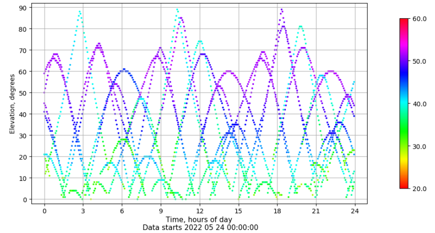
Time-elevation plot for station VIGO. Signal to Noise S1C Data file VIGO00ESP_R_2022144.xtr
