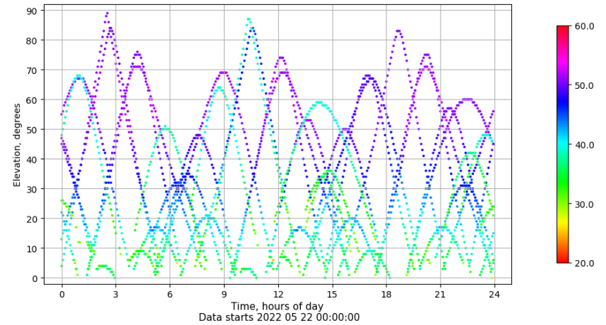
Time-elevation plot for station VIGO. Signal to Noise S1C Data file VIGO00ESP_R_2022142.xtr
