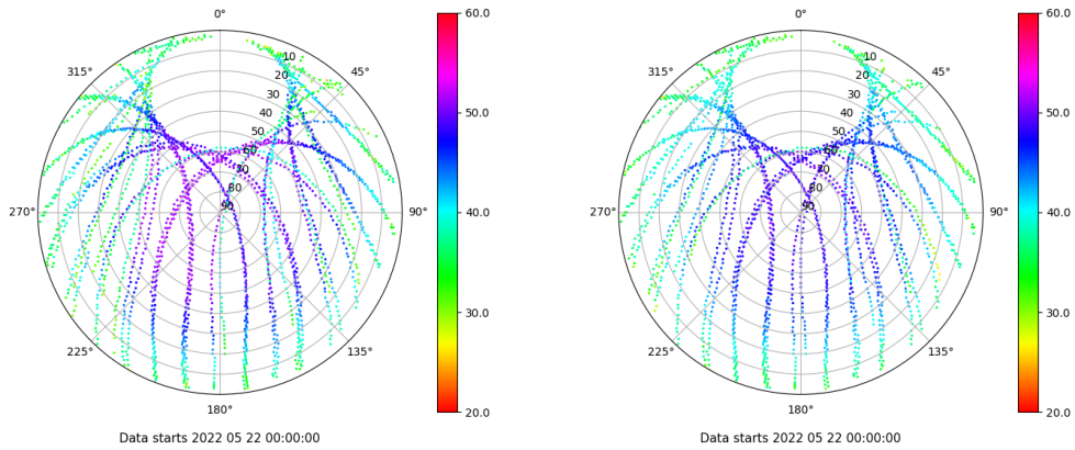
Skyplot for station VIGO. Signal to Noise S1C Data file VIGO00ESP_R_2022142.xtr Skyplot for station VIGO. Signal to Noise S2C Data file VIGO00ESP_R_2022142.xtr
