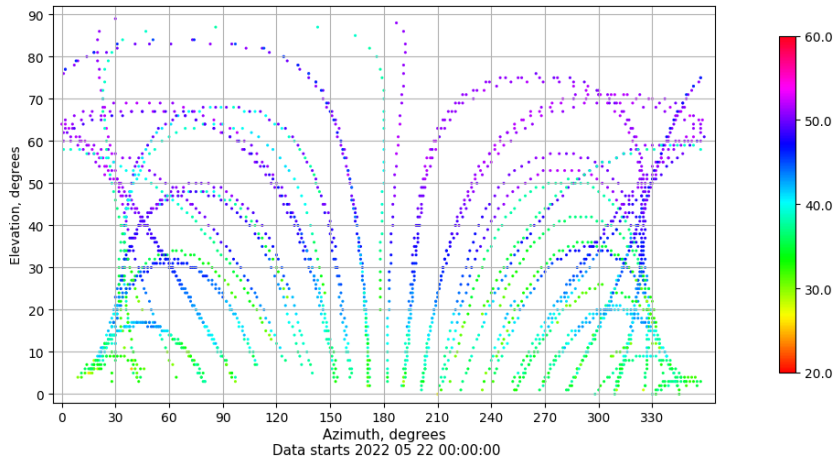
Azimuth-elevation plot for station VIGO. Signal to Noise S1C Data file VIGO00ESP_R_2022142.xtr
