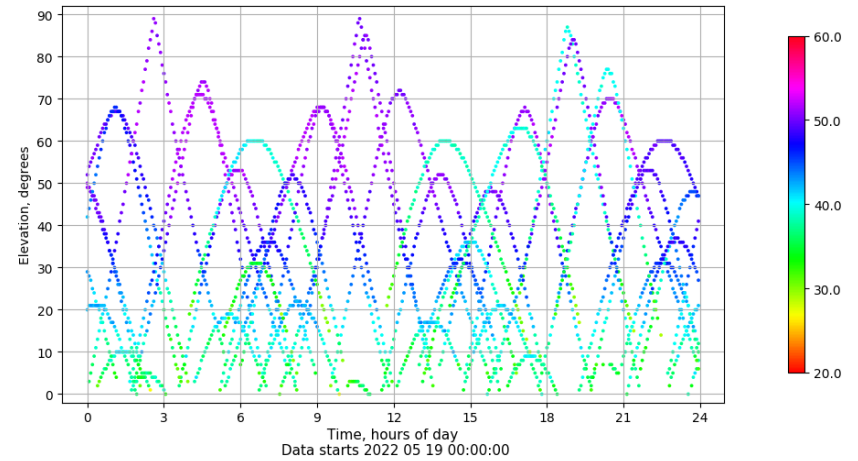
Time-elevation plot for station VIGO. Signal to Noise S1C Data file VIGO00ESP_R_2022139.xtr
