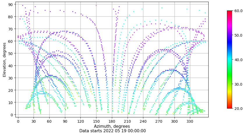
Azimuth-elevation plot for station VIGO. Signal to Noise S1C Data file VIGO00ESP_R_2022139.xtr
