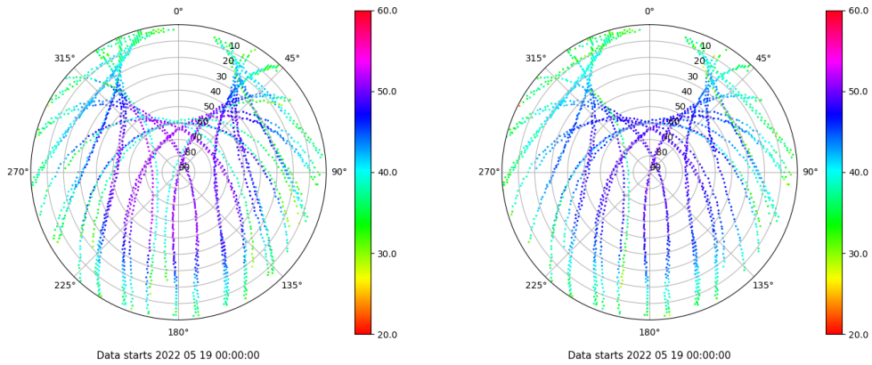
Skyplot for station VIGO. Signal to Noise S1C Data file VIGO00ESP_R_2022139.xtr Skyplot for station VIGO. Signal to Noise S2C Data file VIGO00ESP_R_2022139.xtr
