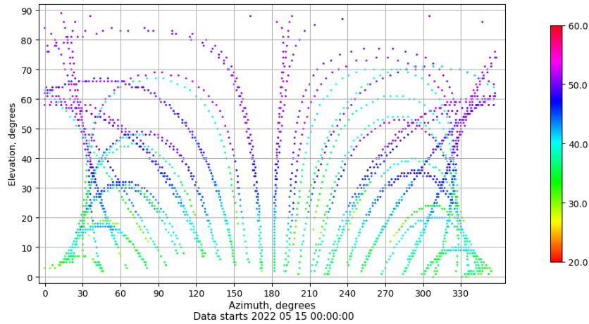
Azimuth-elevation plot for station VIGO. Signal to Noise S1C Data file VIGO00ESP_R_2022135.xtr
