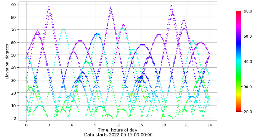
Time-elevation plot for station VIGO. Signal to Noise S1C Data file VIGO00ESP_R_2022135.xtr
