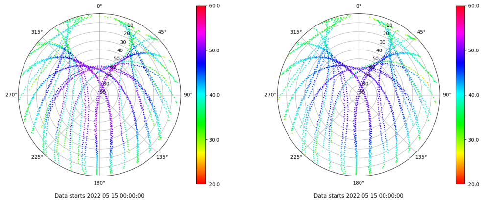
Skyplot for station VIGO. Signal to Noise S1C Data file VIGO00ESP_R_2022135.xtr Skyplot for station VIGO. Signal to Noise S2C Data file VIGO00ESP_R_2022135.xtr
