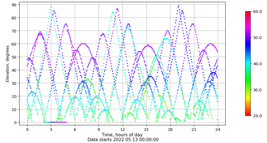
Time-elevation plot for station VIGO. Signal to Noise S1C Data file VIGO00ESP_R_2022133.xtr
