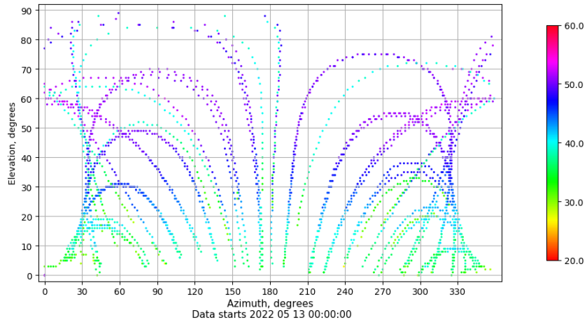
Azimuth-elevation plot for station VIGO. Signal to Noise S1C Data file VIGO00ESP_R_2022133.xtr
