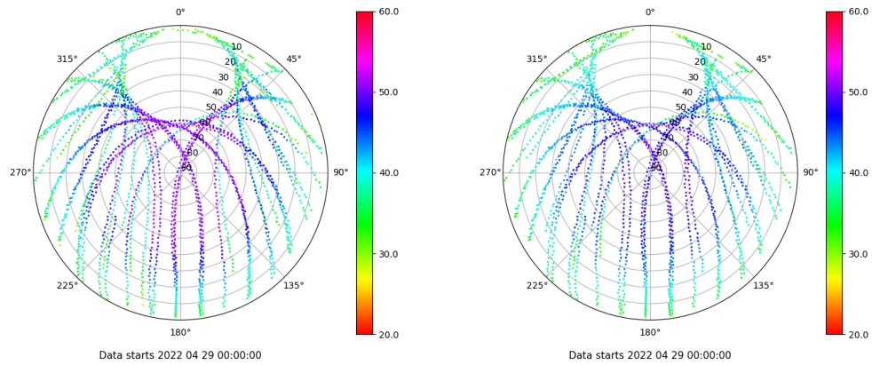
Skyplot for station VIGO. Signal to Noise S1C Data file VIGO00ESP_R_2022119.xtr Skyplot for station VIGO. Signal to Noise S2C Data file VIGO00ESP_R_2022119.xtr
