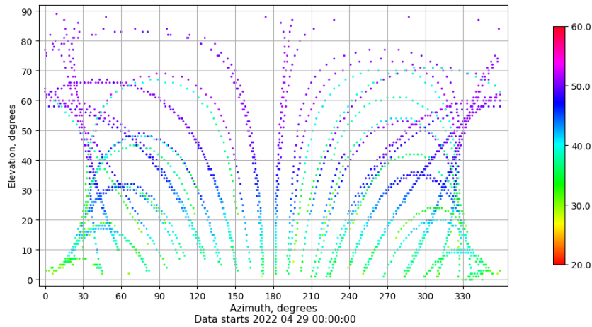
Azimuth-elevation plot for station VIGO. Signal to Noise S1C Data file VIGO00ESP_R_2022119.xtr
