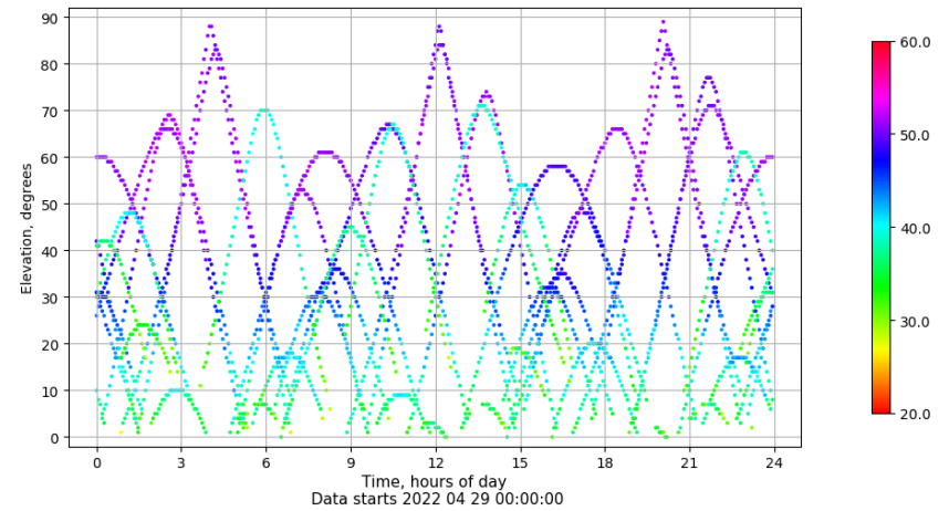
Time-elevation plot for station VIGO. Signal to Noise S1C Data file VIGO00ESP_R_2022119.xtr
