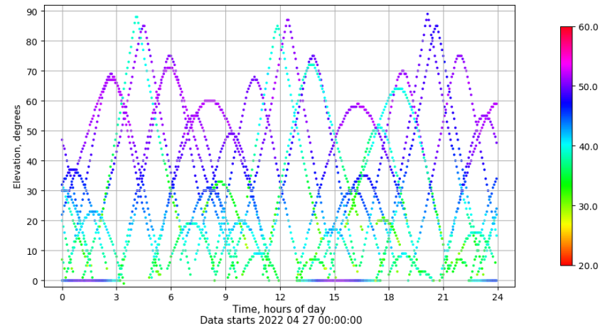
Time-elevation plot for station VIGO. Signal to Noise S1C Data file VIGO00ESP_R_2022117.xtr
