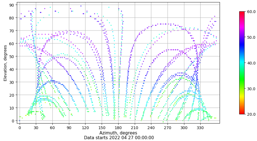
Azimuth-elevation plot for station VIGO. Signal to Noise S1C Data file VIGO00ESP_R_2022117.xtr
