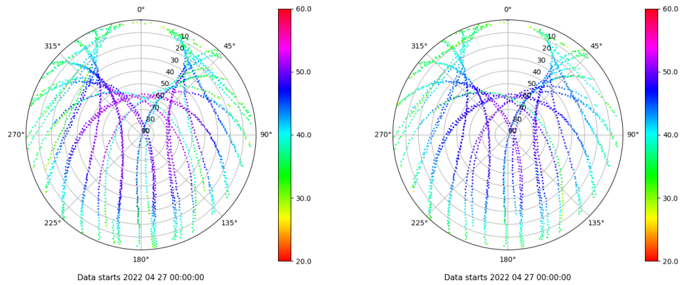
Skyplot for station VIGO. Signal to Noise S1C Data file VIGO00ESP_R_2022117.xtr Skyplot for station VIGO. Signal to Noise S2C Data file VIGO00ESP_R_2022117.xtr
