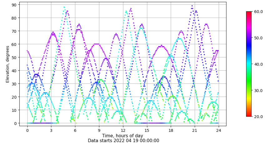
Time-elevation plot for station VIGO. Signal to Noise S1C Data file VIGO00ESP_R_2022109.xtr
