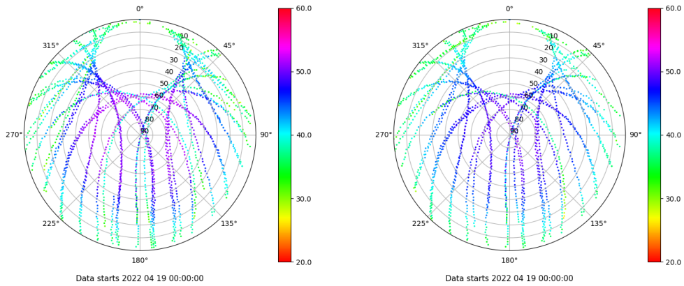
Skyplot for station VIGO. Signal to Noise S1C Data file VIGO00ESP_R_2022109.xtr Skyplot for station VIGO. Signal to Noise S2C Data file VIGO00ESP_R_2022109.xtr
