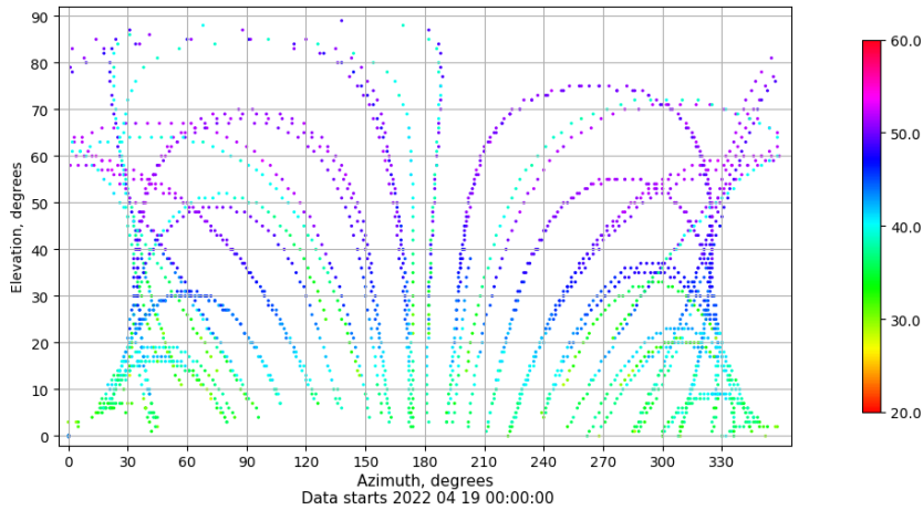
Azimuth-elevation plot for station VIGO. Signal to Noise S1C Data file VIGO00ESP_R_2022109.xtr
