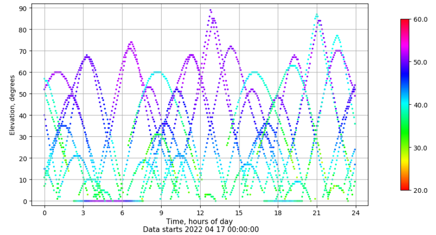
Time-elevation plot for station VIGO. Signal to Noise S1C Data file VIGO00ESP_R_2022107.xtr
