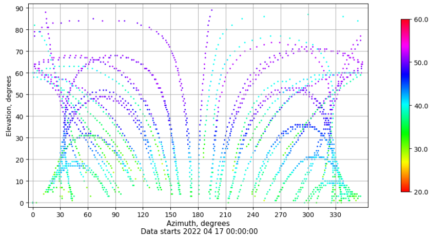
Azimuth-elevation plot for station VIGO. Signal to Noise S1C Data file VIGO00ESP_R_2022107.xtr
