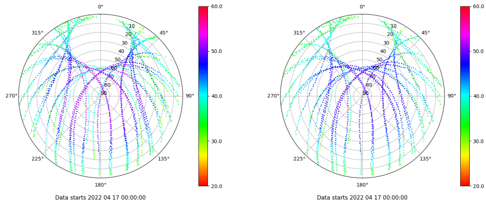
Skyplot for station VIGO. Signal to Noise S1C Data file VIGO00ESP_R_2022107.xtr Skyplot for station VIGO. Signal to Noise S2C Data file VIGO00ESP_R_2022107.xtr
