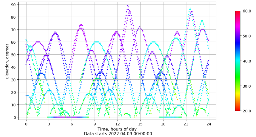
Time-elevation plot for station VIGO. Signal to Noise S1C Data file VIGO00ESP_R_2022099.xtr
