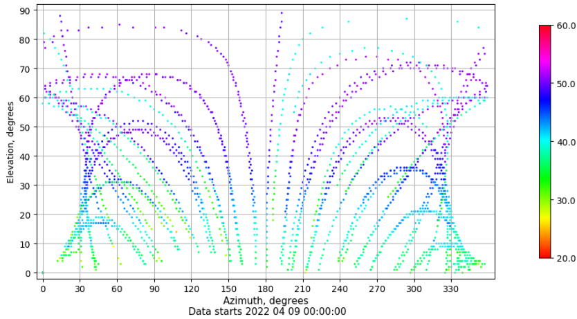
Azimuth-elevation plot for station VIGO. Signal to Noise S1C Data file VIGO00ESP_R_2022099.xtr
