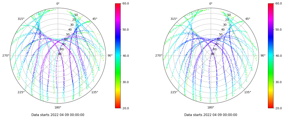
Skyplot for station VIGO. Signal to Noise S1C Data file VIGO00ESP_R_2022099.xtr Skyplot for station VIGO. Signal to Noise S2C Data file VIGO00ESP_R_2022099.xtr
