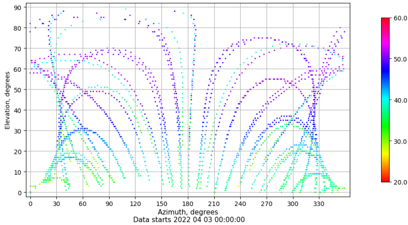
Azimuth-elevation plot for station VIGO. Signal to Noise S1C Data file VIGO00ESP_R_2022093.xtr
