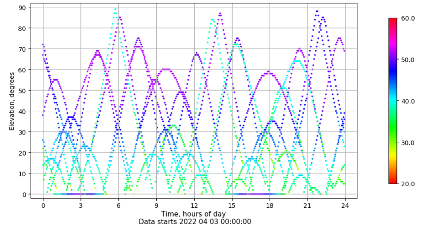
Time-elevation plot for station VIGO. Signal to Noise S1C Data file VIGO00ESP_R_2022093.xtr
