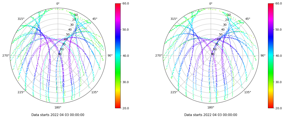
Skyplot for station VIGO. Signal to Noise S1C Data file VIGO00ESP_R_2022093.xtr Skyplot for station VIGO. Signal to Noise S2C Data file VIGO00ESP_R_2022093.xtr
