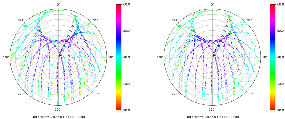
Skyplot for station VIGO. Signal to Noise S1C Data file VIGO00ESP_R_2022090.xtr Skyplot for station VIGO. Signal to Noise S2C Data file VIGO00ESP_R_2022090.xtr
