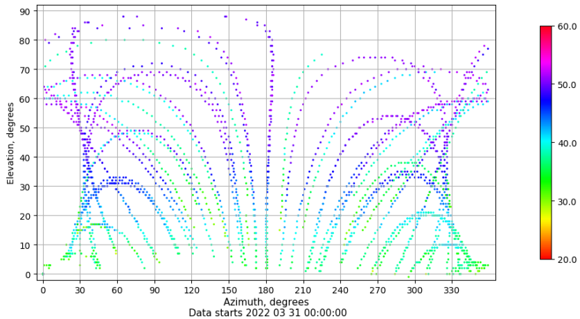
Azimuth-elevation plot for station VIGO. Signal to Noise S1C Data file VIGO00ESP_R_2022090.xtr
