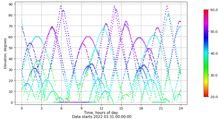
Time-elevation plot for station VIGO. Signal to Noise S1C Data file VIGO00ESP_R_2022090.xtr
