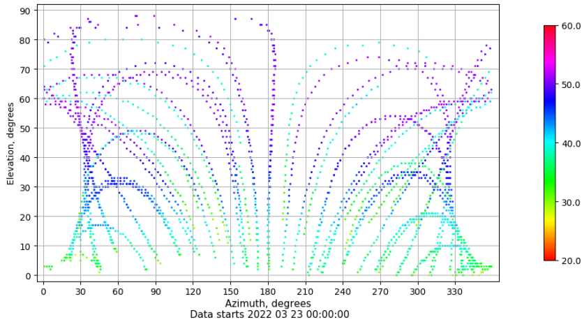
Azimuth-elevation plot for station VIGO. Signal to Noise S1C Data file VIGO00ESP_R_2022082.xtr
