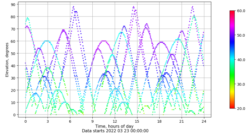
Time-elevation plot for station VIGO. Signal to Noise S1C Data file VIGO00ESP_R_2022082.xtr
